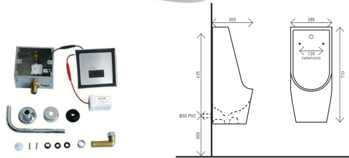
Urínol COM SENSOR S300/420 Ref.: RSU3032SS
